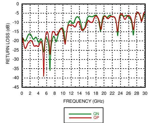
Output Return Loss vs. Frequency [1][4]
